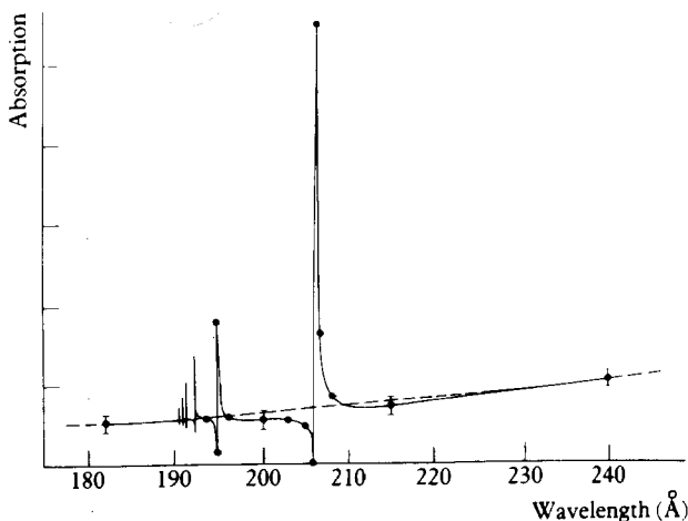
6.9 Resonances found in the continuous absorption spectrum of helium by R. B. Madden and K. Codling.
